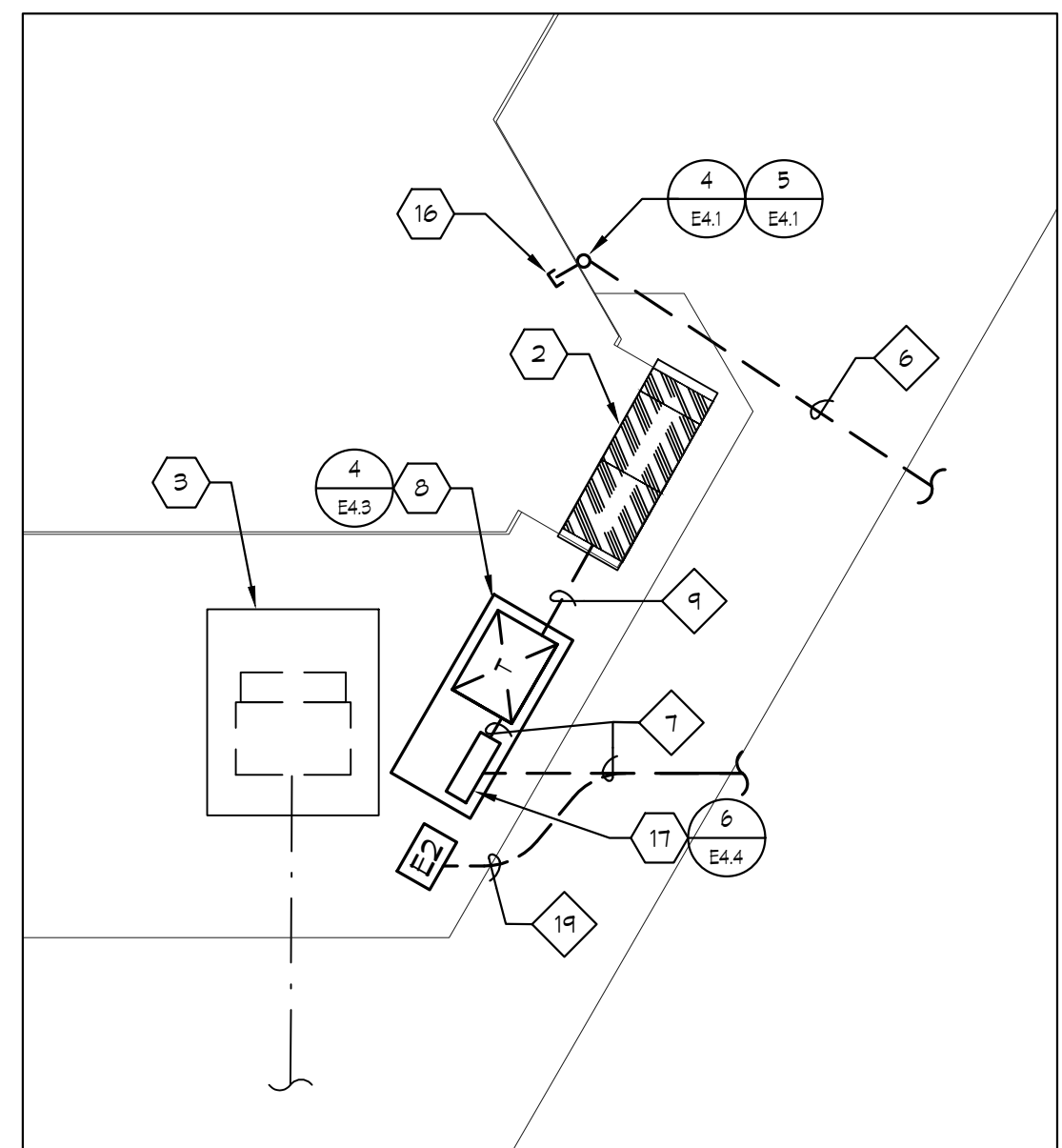
ELECTRICAL SWITCHGEAR DIMENSIONS SCALE: 1/8"=1'-0"
