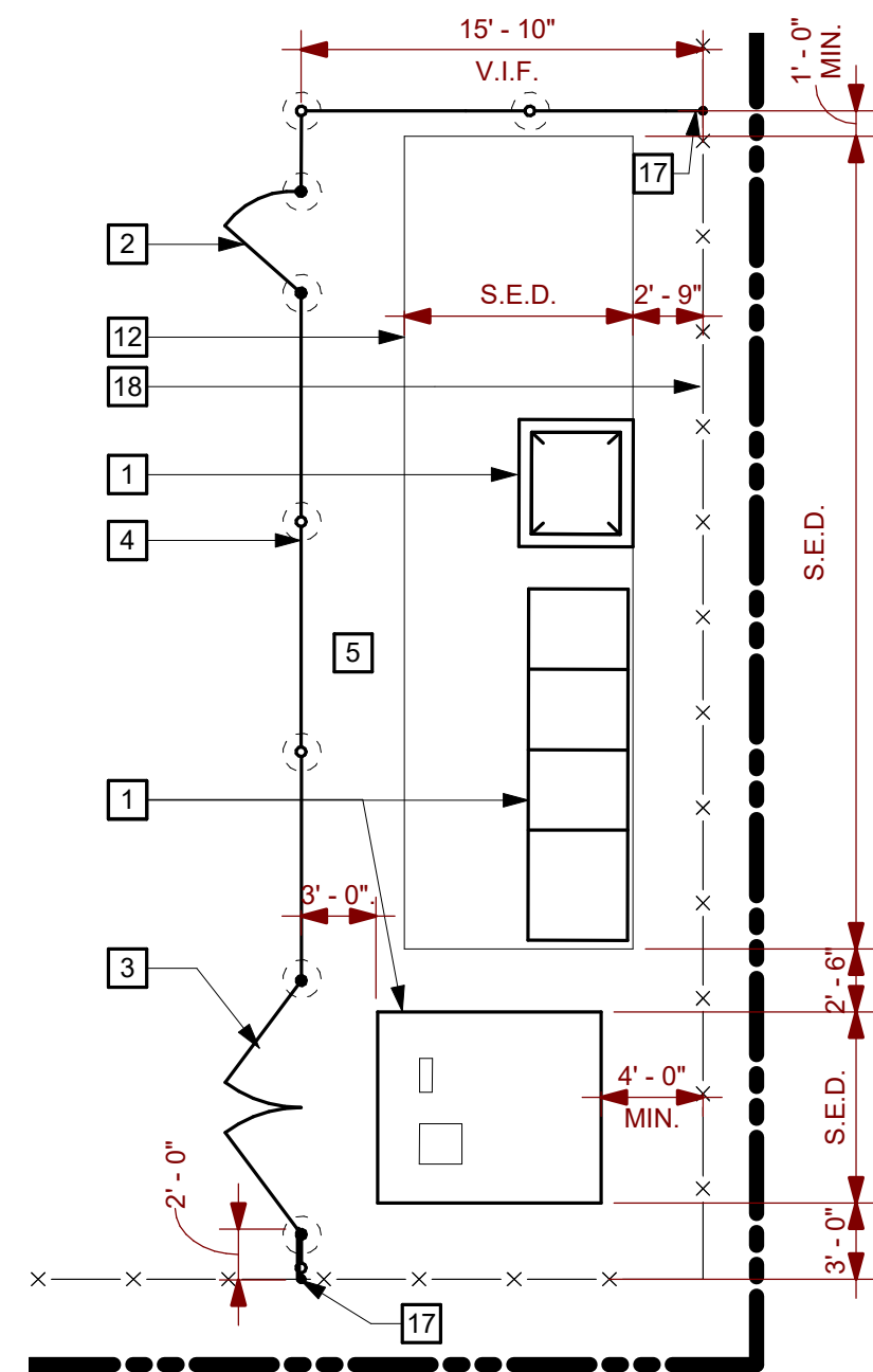
2 ENLARGED SITE PLAN SCALE: 1/8" = 1'-0"
