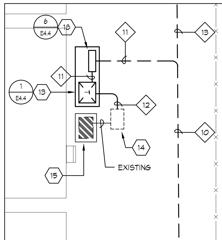
ENLARGED SITE PLAN SCALE: 1/8"=1'-0"
