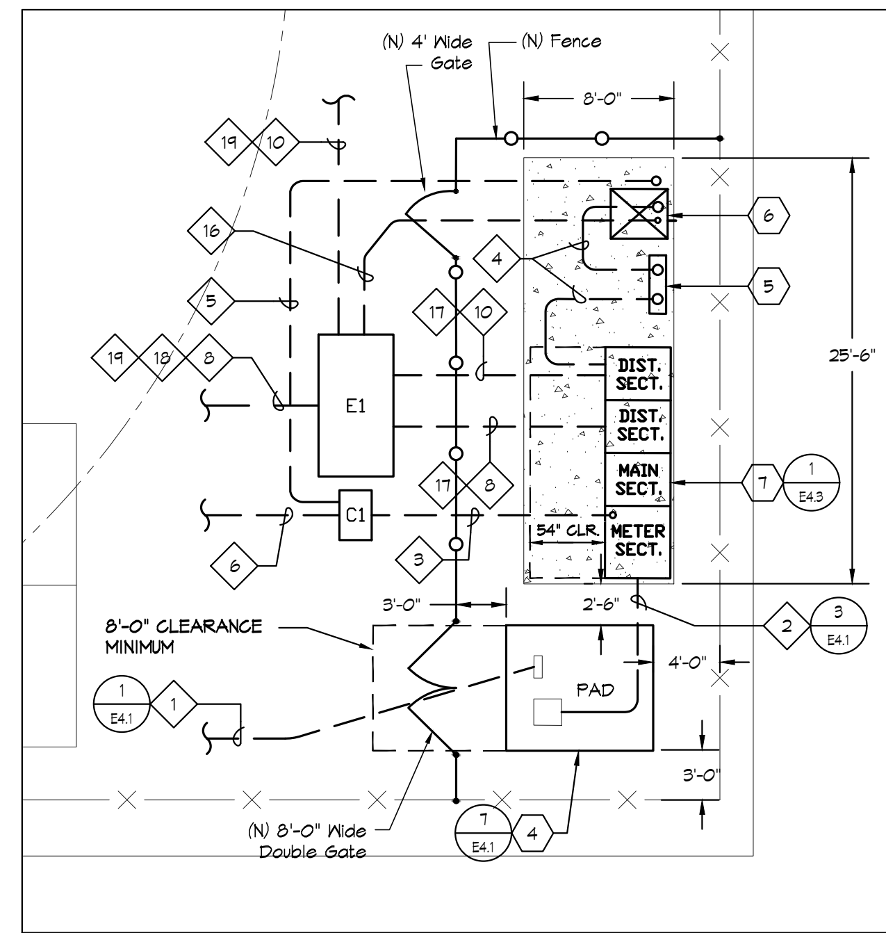
ELECTRICAL SWITCHGEAR DIMENSIONS SCALE: 1/8"=1'-0"
